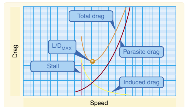
Figure 10-5. Drag versus speed.
