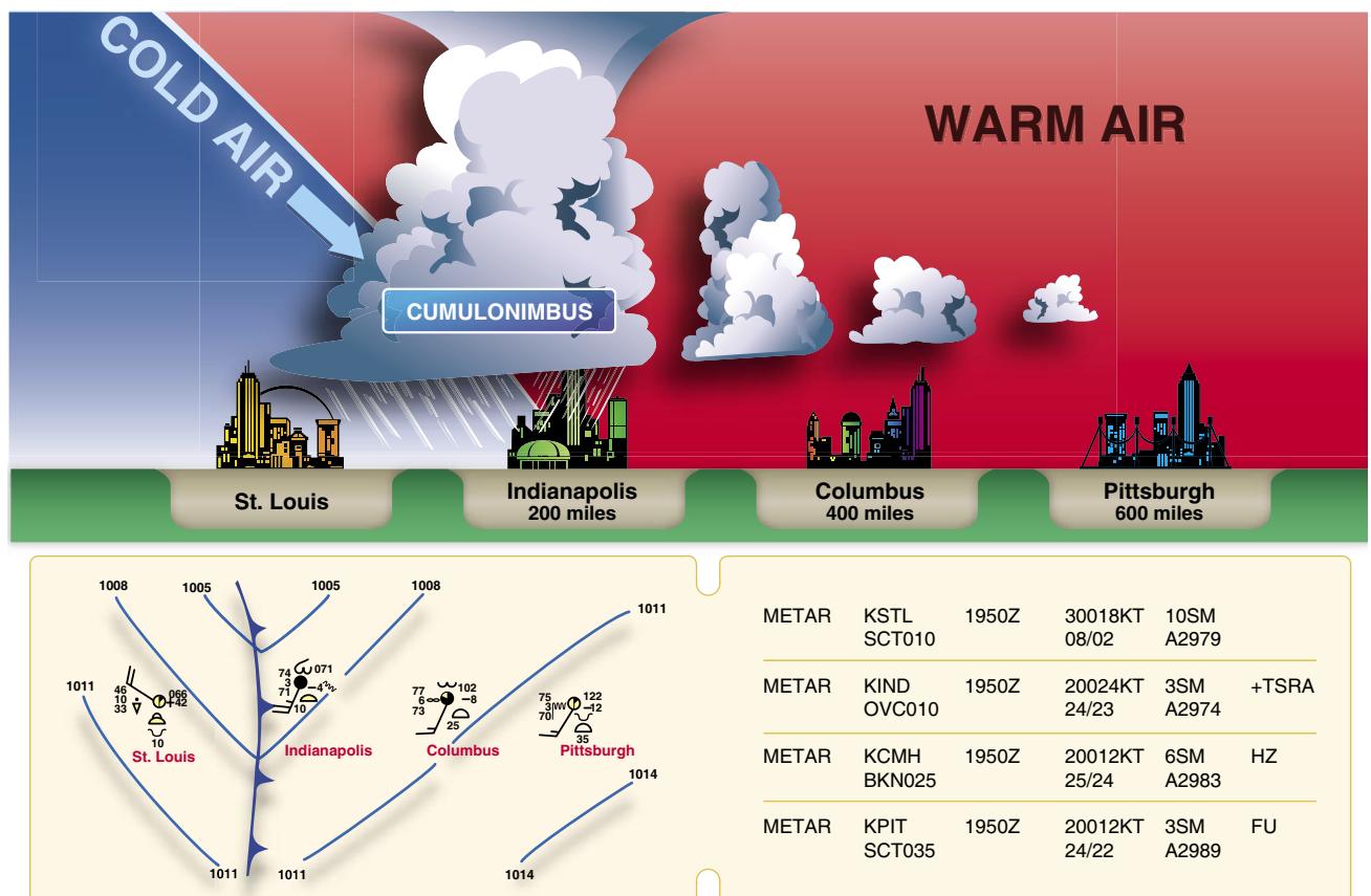
Figure 11-27. Cold front cross-section with surface weather chart depiction and associated METAR.
