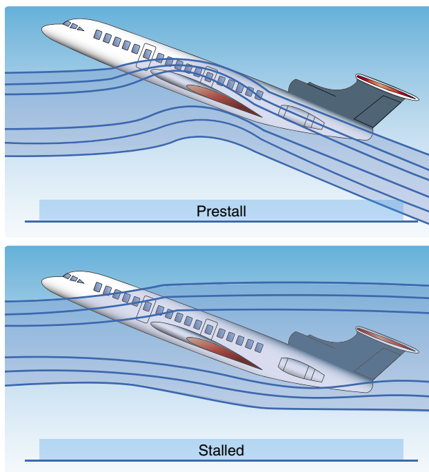
Figure 4-62. T-tail stall.
