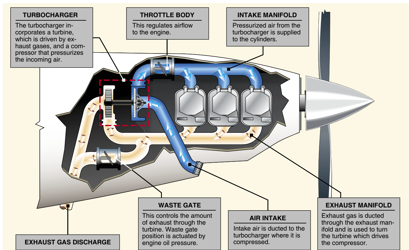
Figure 6-15. Turbocharger components.
