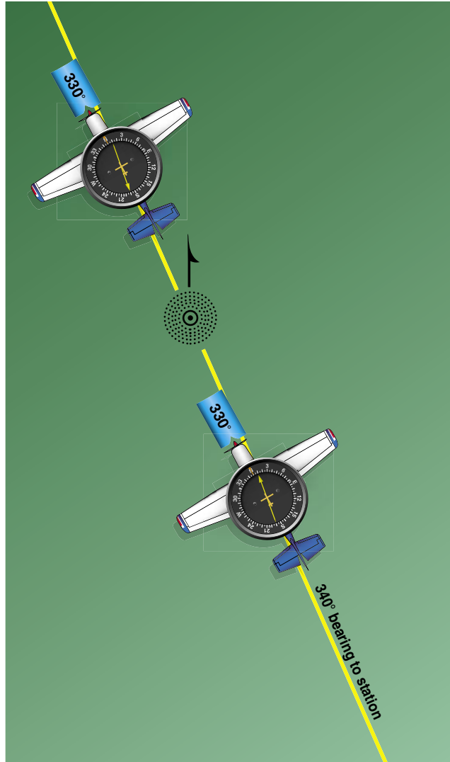
Figure 15-38. ADF tracking.
