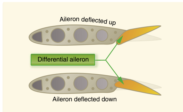
Figure 5-6. Differential ailerons.
