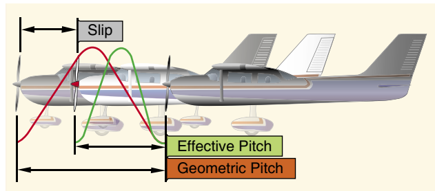
Figure 4-37. Propeller slipage.
