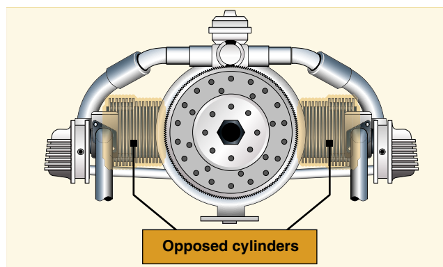
Figure 6-2. Horizontally opposed engine.
