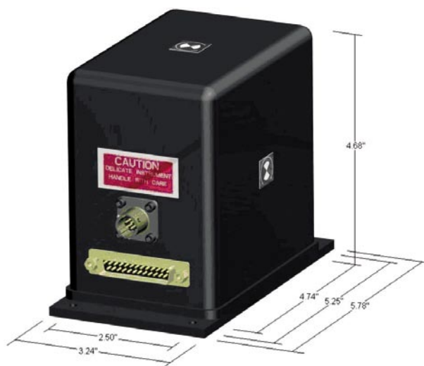
Figure 7-26. Attitude and heading reference system (AHRS).
