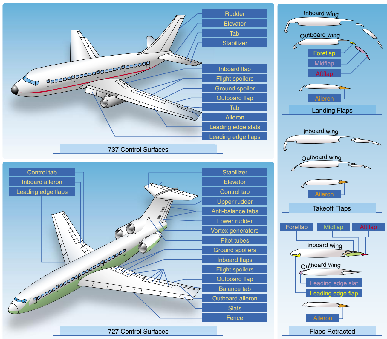
Figure 4-63. Control surfaces.
