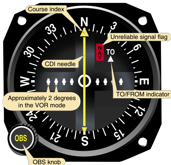
Figure 15-29. VOR indicator.
