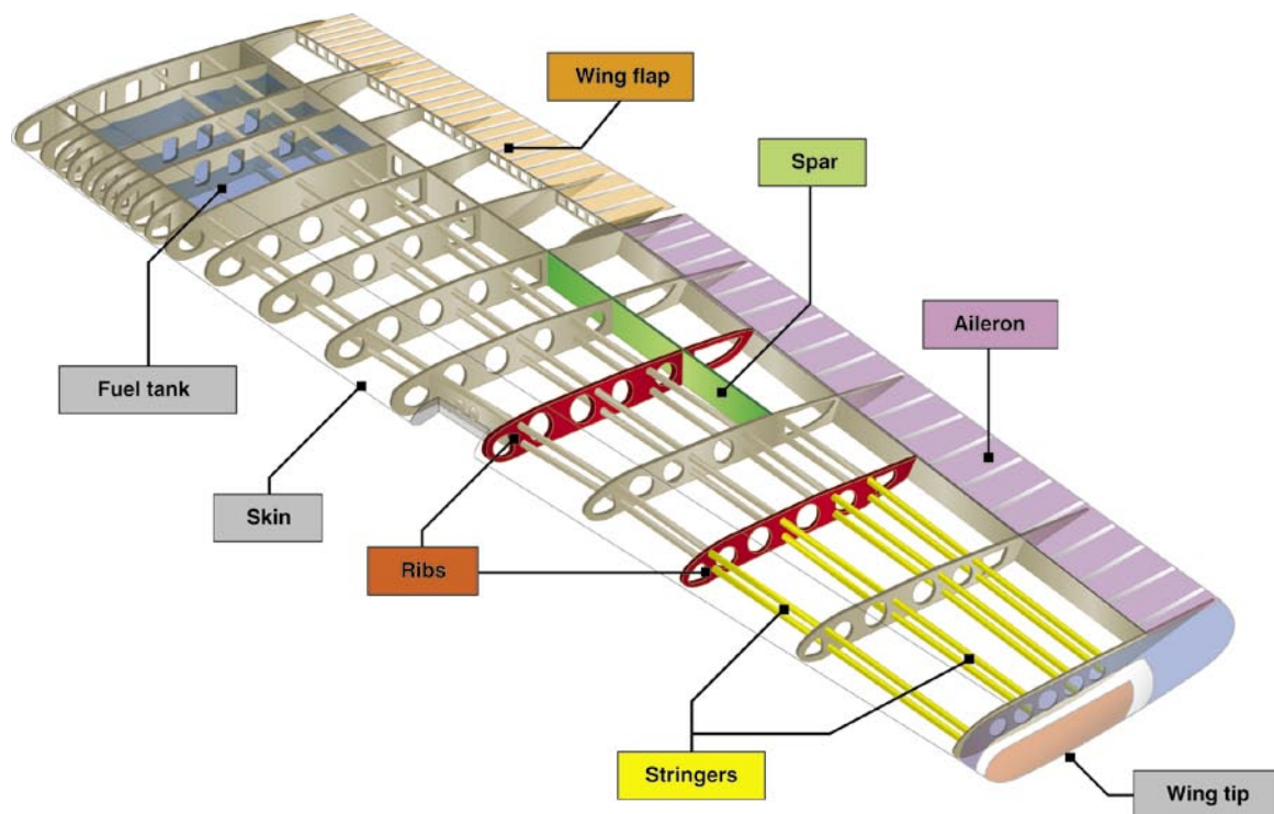
Figure 2-7. Wing components.
