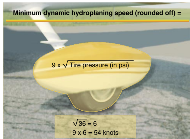
Figure 10-17. Tire pressure.
