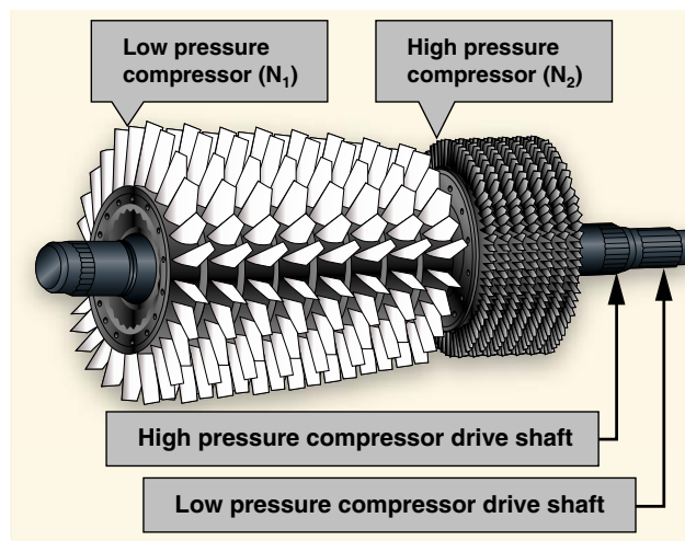
Figure 6-27. Dual-spool axial-flow compressor.
