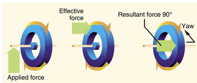
Figure 4-41. Gyroscopic precession.
