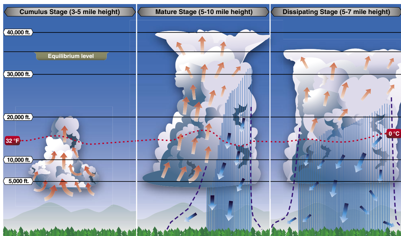
Figure 11-23. Life cycle of a thunderstorm.
