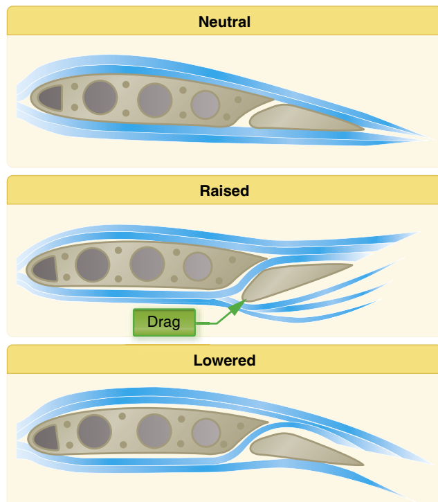
Figure 5-7. Frise-type ailerons.
