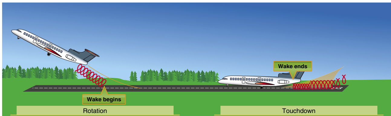
Figure 13-21. Vortex behavior.
