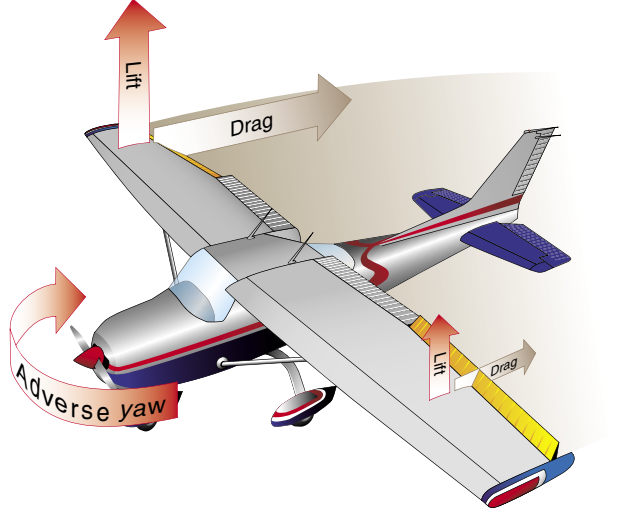
Figure 5-5. Adverse yaw is caused by higher drag on the outside wing, which is producing more lift.
