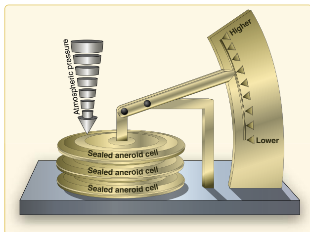
Figure 11-7. Aneroid barometer.
